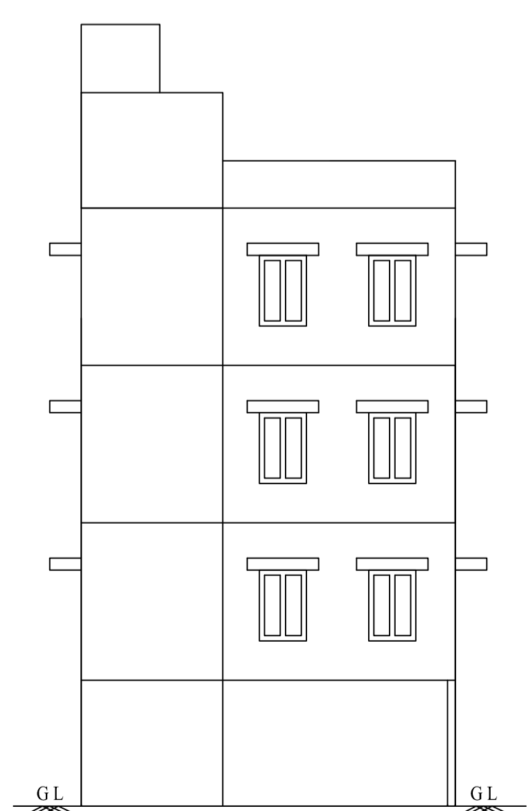
FRONT ELEVATION
