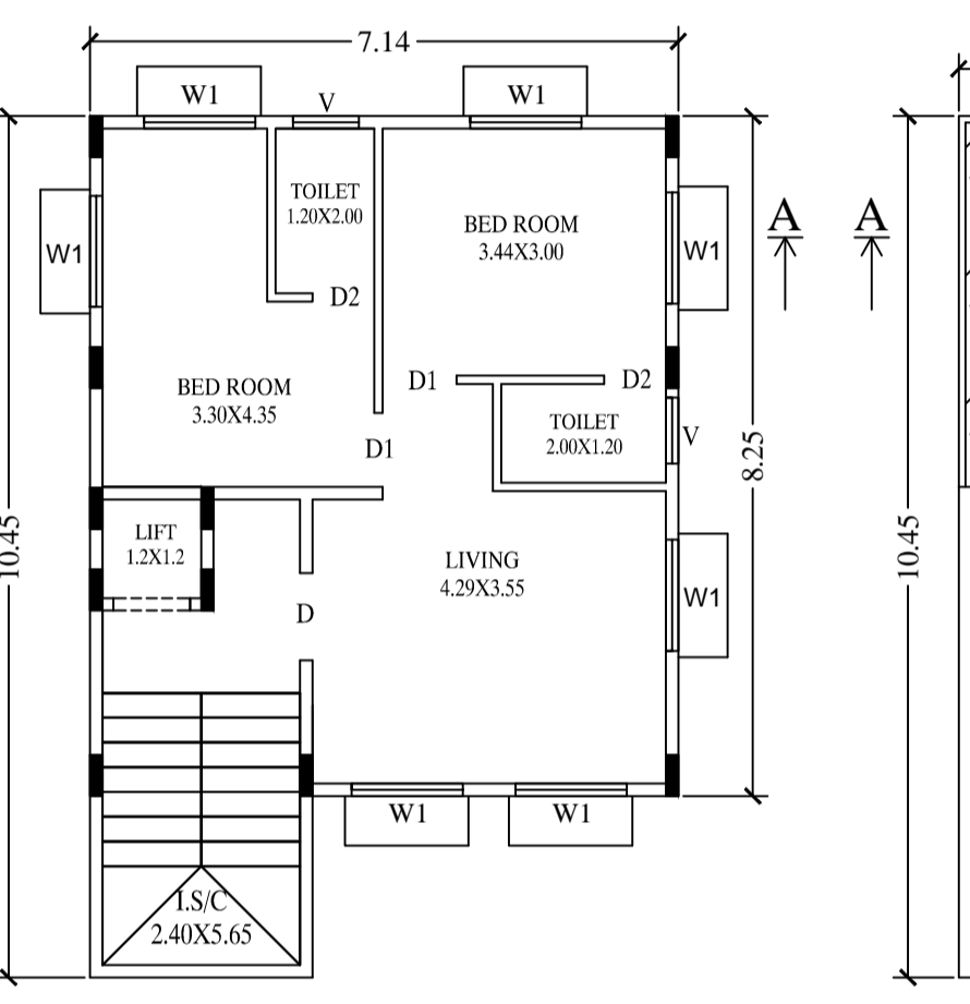
PROPOSED TYPICAL 1ST AND 2ND FLOOR PLAN
